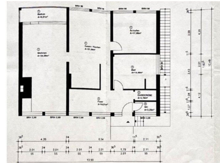
Grundriss WHG 1
