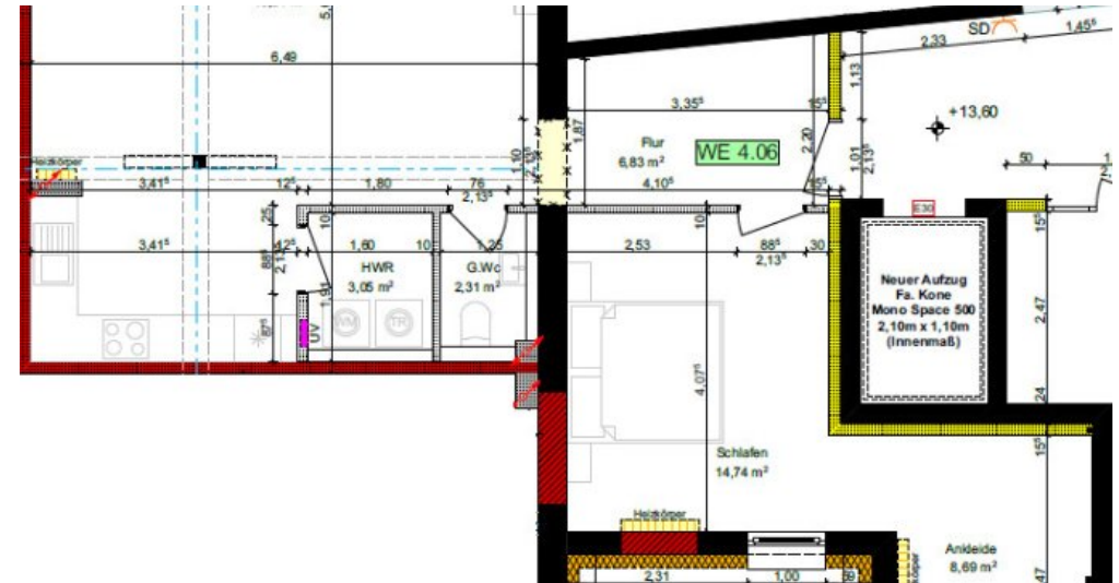
Grundriss WHG 4.06
